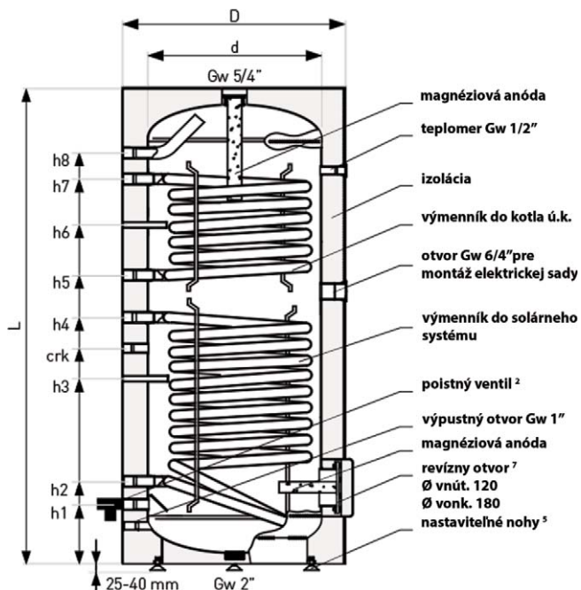
QUADROFLEX QFS 2P / 400
