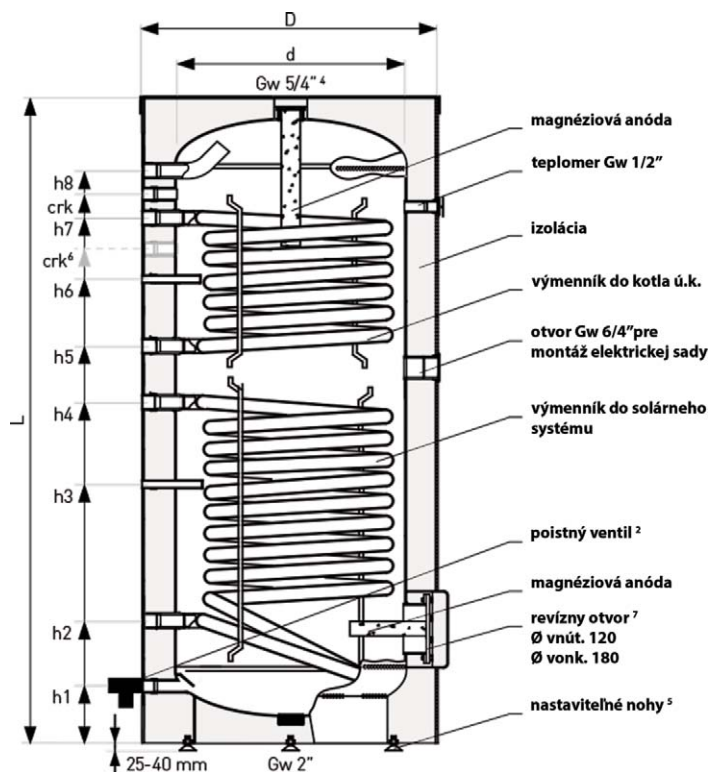
QUADROFLEX QFS 2P / 500 - 1500
