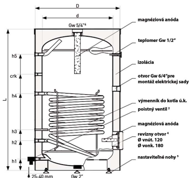
QUADROFLEX QFS 1P / 500 - 1500
