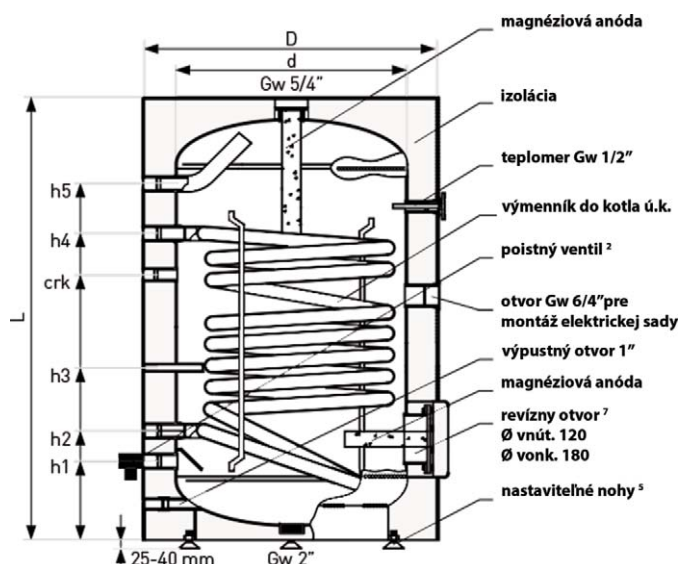
QUADROFLEX QFS 1P / 200 - 400
